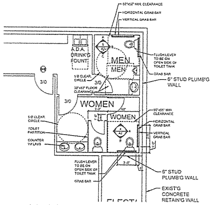
③ LARGE SCALE TOILET ROOM PLAN SCALE: 1/4"=1'-0"
