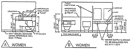
④ TOILET ROOM INTERIOR ELEVATIONS SCALE: 1/4"=1'-0"
