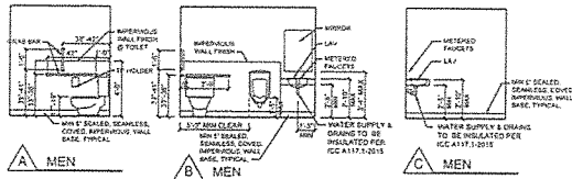
⑤ TOILET ROOM INTERIOR ELEVATIONS SCALE: 1/4"=1'-0"
