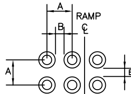
DETECTABLE WARNING PATTERN DETAIL TRUNCATED DOMES
