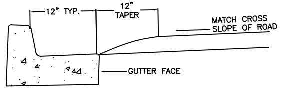
SECTION B-B TAPER TO CURB AND GUTTER
