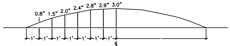
SECTION A-A PARABOLIC CROWN
