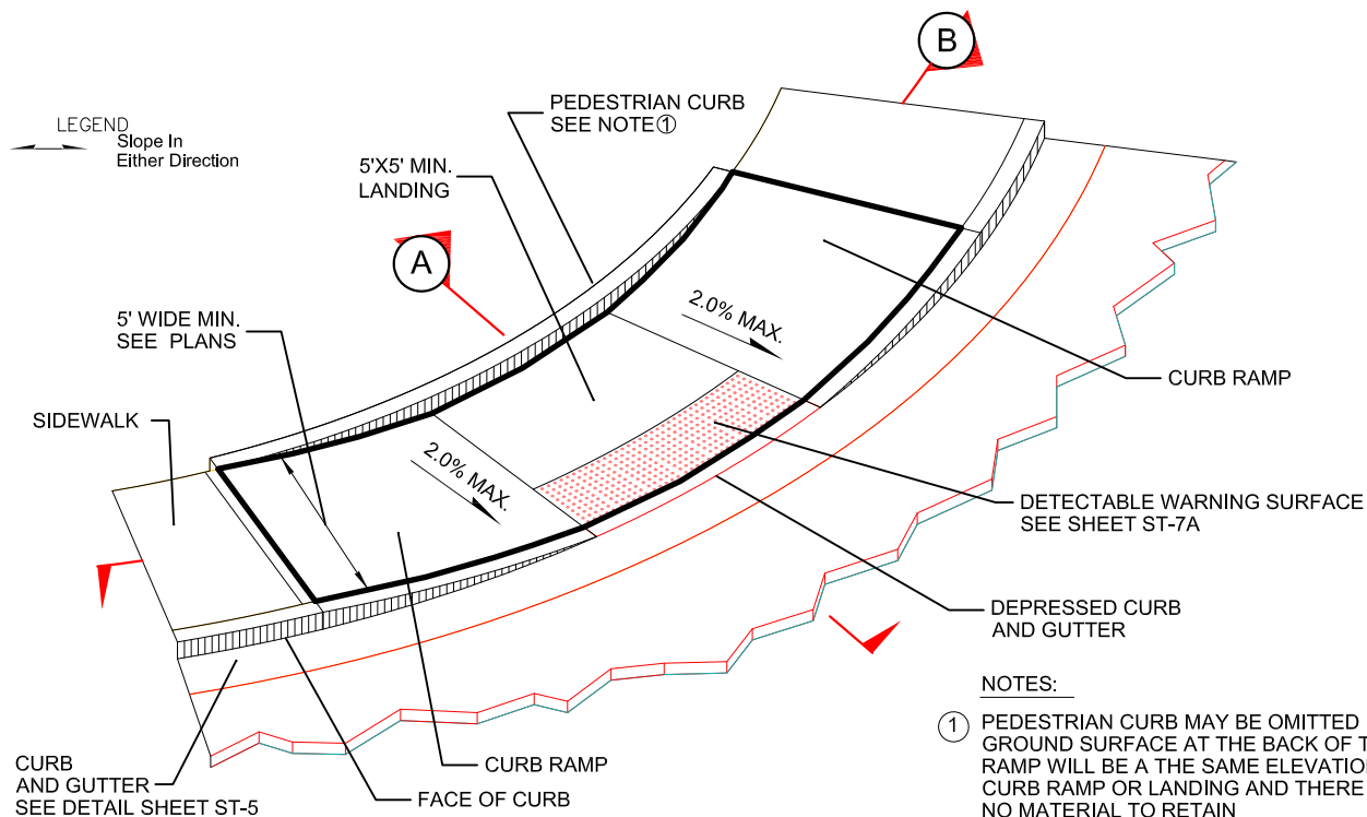
ISOMETRIC VIEW
