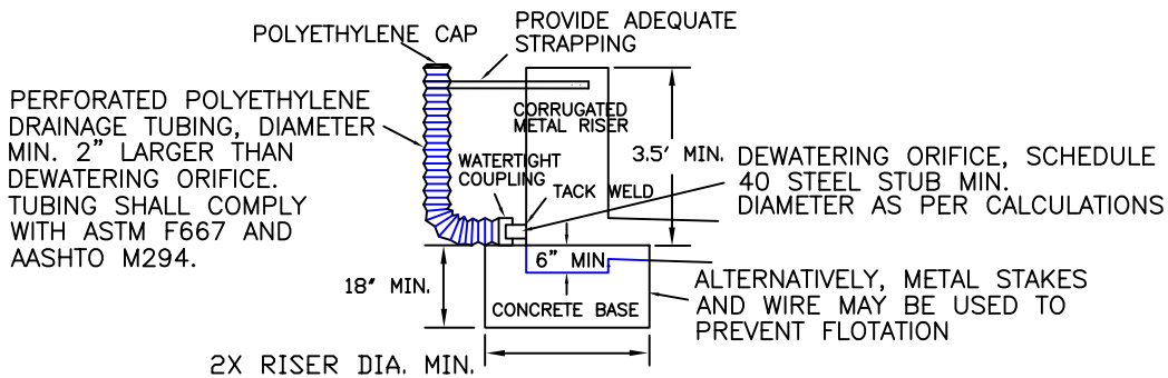
RISER DETAIL
