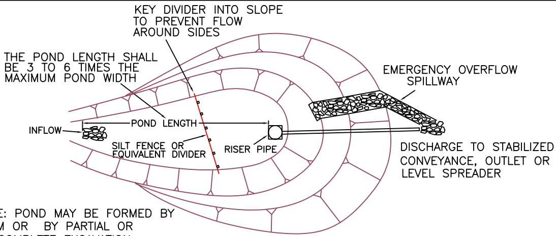
PLAN VIEW
