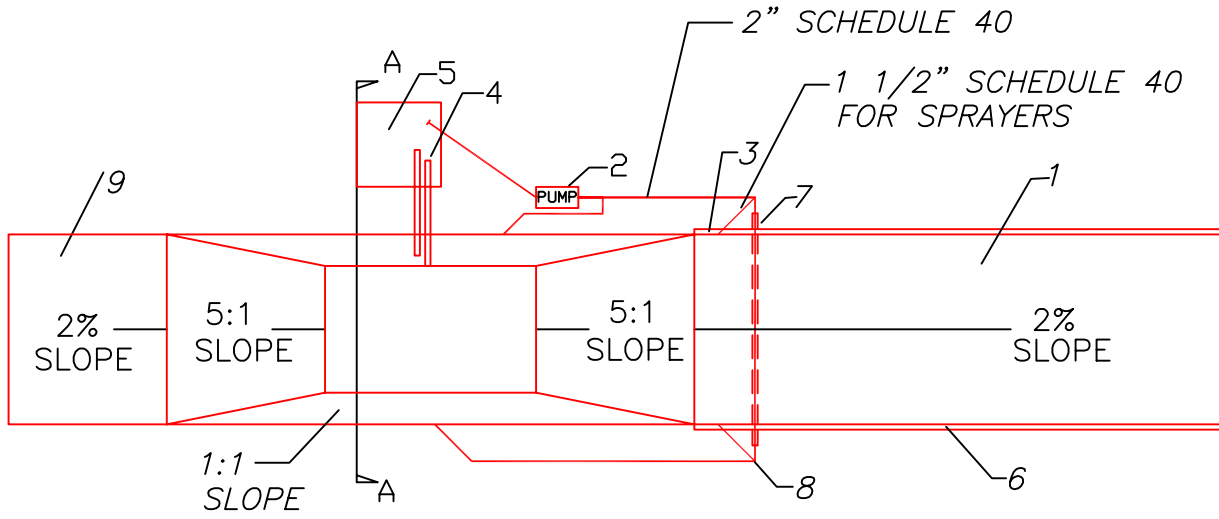
WHEEL WASH PLAN
