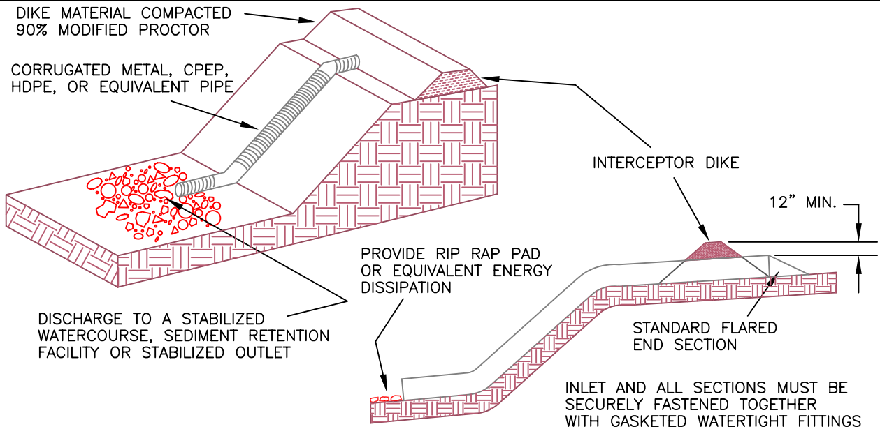
PIPE SLOPE DRAIN
