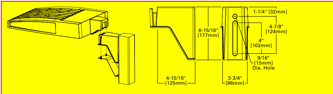
QM Quick Mount Arm (Standard)
