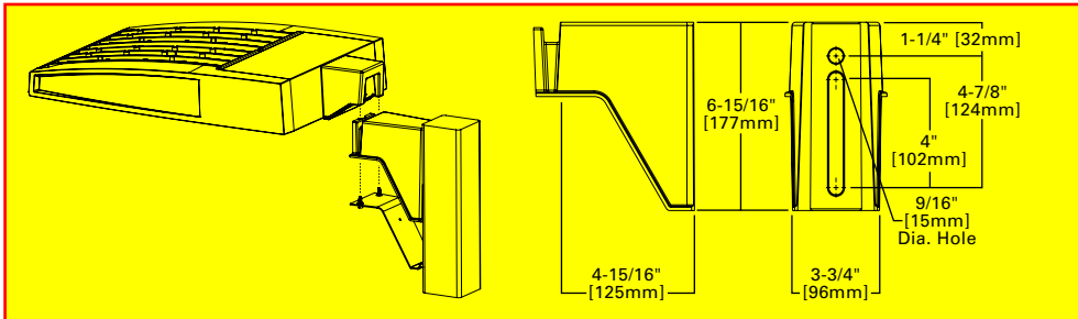
QM Quick Mount Arm (Standard)
