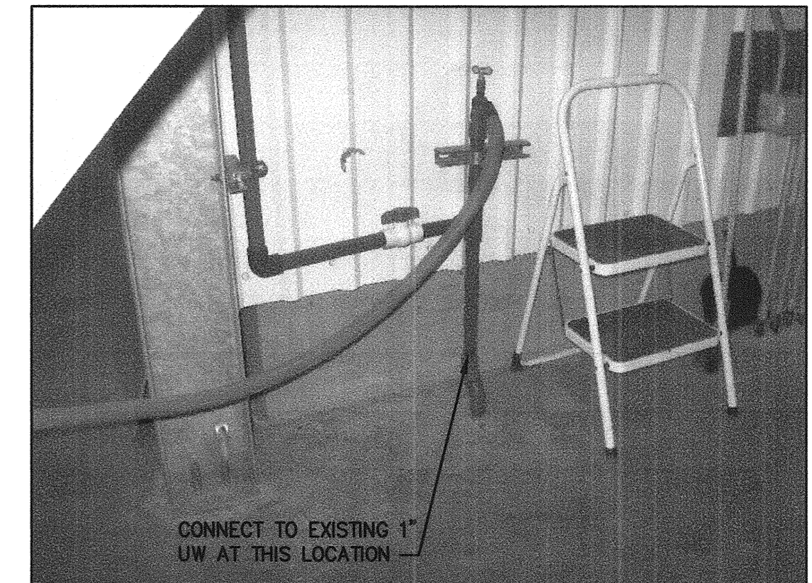
1 BIOSOLIDS HANDLING BLDG UW CONNECTION C104 SCALE: NTS
